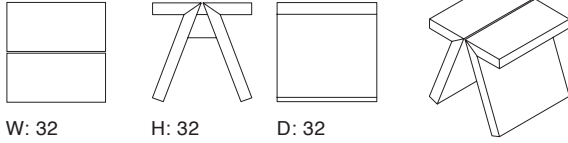
SUPERSOLID Object 1
