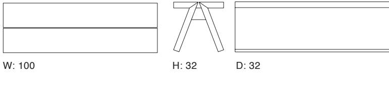
SUPERSOLID Object 3
