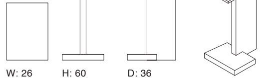
SUPERSOLID Object 5
