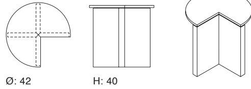
SUPERSOLID Object 2
